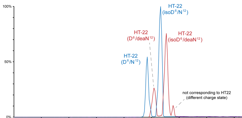
Figure 6. Extracted ion electropherograms of m/z values corresponding to different forms of synthetic peptides HT-22 spiked in Universal Proteomic Standard 1 peptide mixture analyzed by sheathless capillary zone electrophoresis–electrospray ionization–MS/MS.
