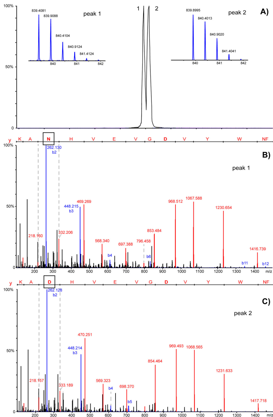
Figure 2. (a) Extracted ion electropherograms for the m/z values corresponding to peptide HT-22 and peptide HT-22 (deaN 12 ) with MS isotopic profiles corresponding to each peak. (b) MS/MS spectrum corresponding to peptide HT-22. (c) MS/MS spectrum corresponding to peptide HT-22 (deaN 12 ).
