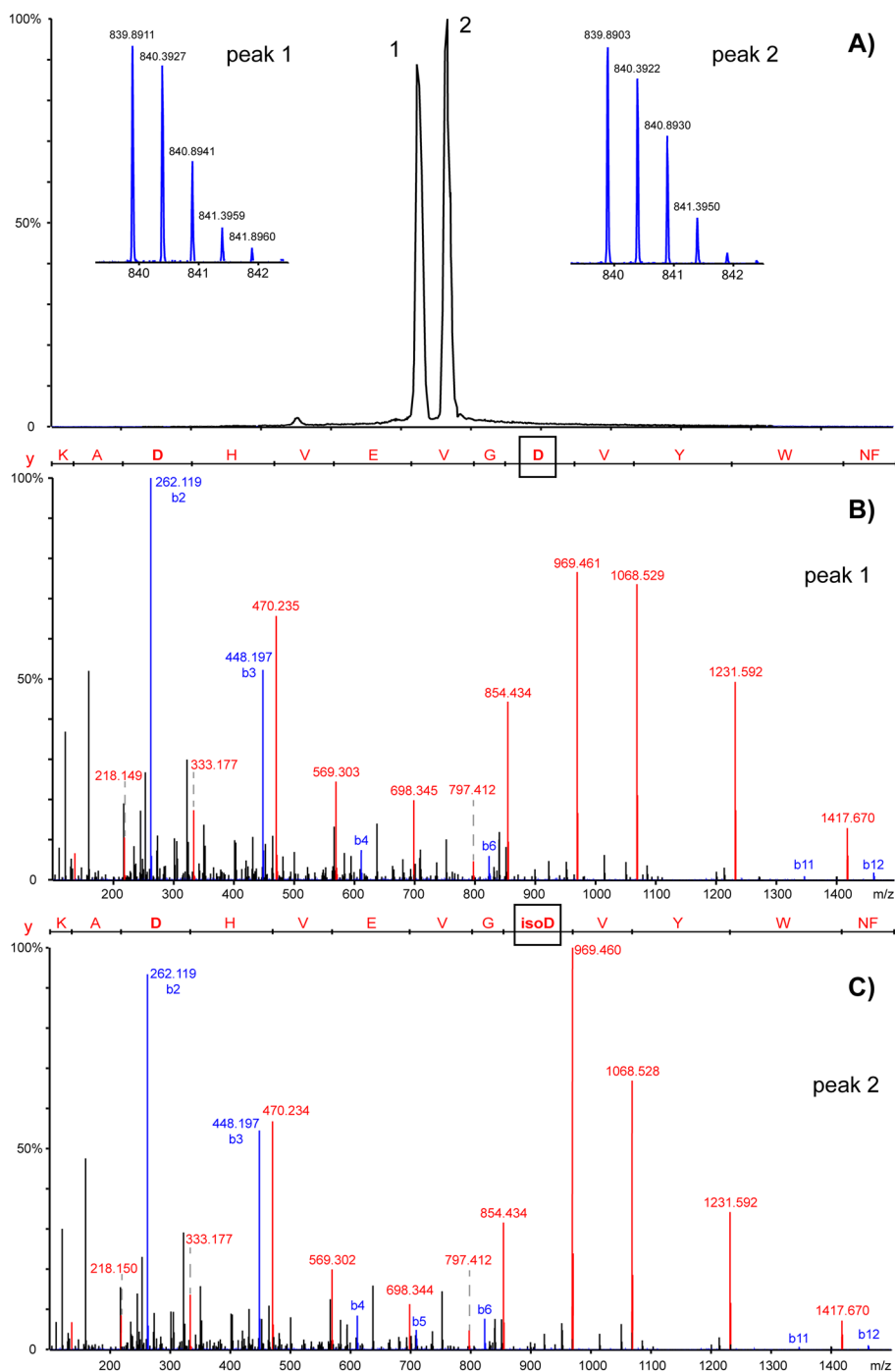
Figure 3. (a) Extracted ion electropherograms of m/z value corresponding to peptide HT-22 (D 6 /deaN 12 ) and peptide HT-22 (isoD 6 /deaN 12 ) with MS isotopic profiles corresponding to each peak. (b) MS/MS spectrum corresponding to peptide HT-22 (D 6 /deaN 12 ). (c) MS/MS spectrum corresponding to peptide HT-22 (isoD 6 /deaN 12 ).
