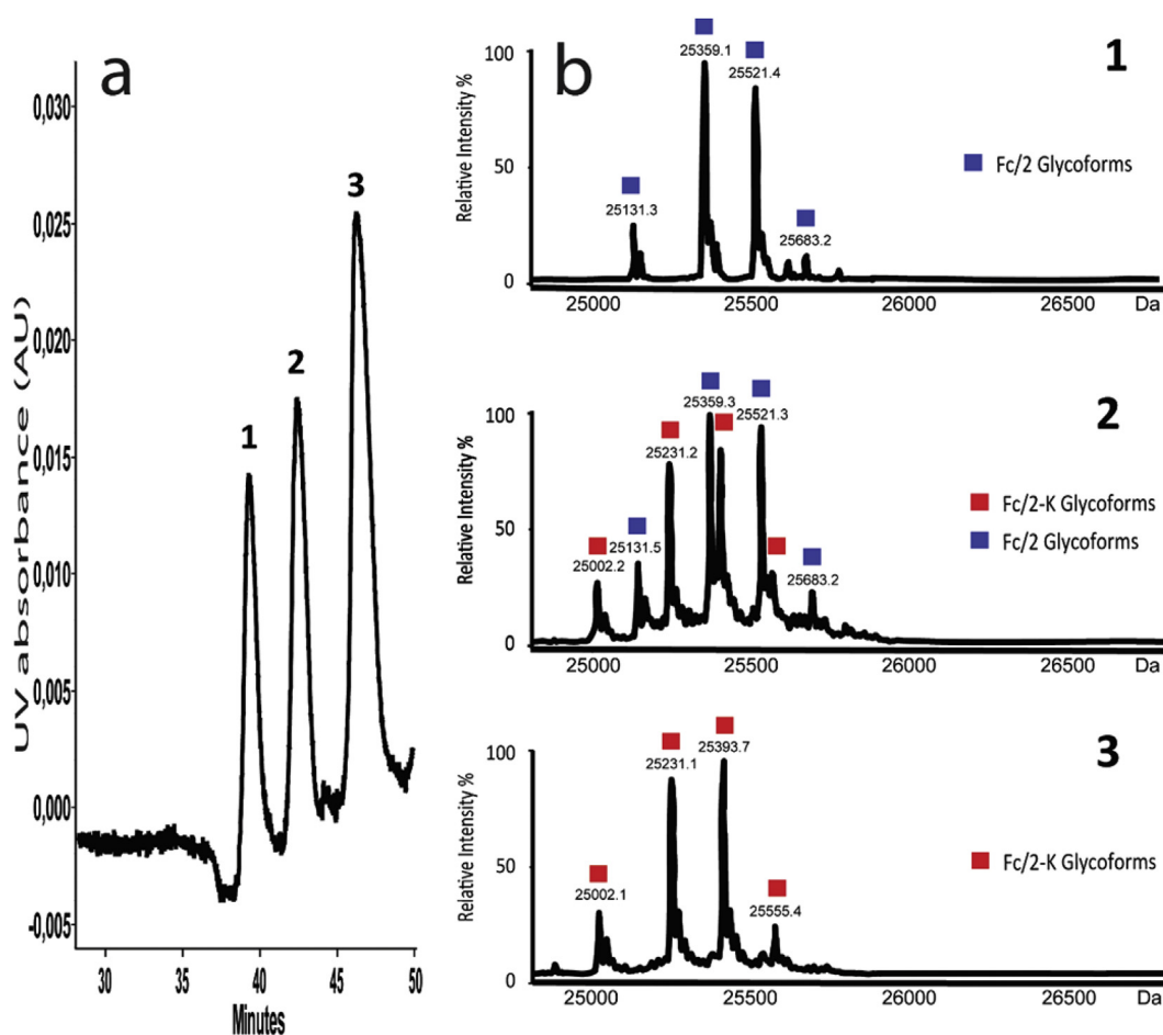
Fig. 1. (a) Off line CZE-UV/ESI-MS separation of middle-up cetuximab charge variants. (b) Deconvoluted mass spectra for each F_{c/2} variant. The MS peak were labeled with the correspondent glycoform. Experimental conditions: Inlet BGE: EACA 200 mM ammonium acetate 25 mM pH 5.70 and outlet BGE: ammonium acetate 25 mM pH 5.70; HPC-coated capillary, total/effective length 82/75.5 cm \times 75 \mu m i.d.; voltage, 20 kV; UV absorbance at 200 nm; MS condition: See Experimental section; sample, IdeS digest of cetuximab (5 \mu g/ \mu L); sample injection 0.5 psi 50s.
