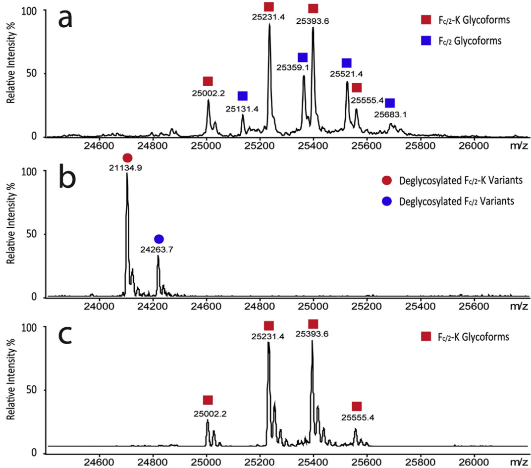
Fig. 4. Fc 1/2 variants deconvoluted mass spectra of (a) IdeS digest cetuximab, (b) IgGZERO + IdeS digest cetuximab and (c) CP-B + IdeS digest cetuximab. Experimental conditions: 50%/49%/1%, acetonitrile/water/formic acid (v/v/v); sample concentration 1 \mu M.
