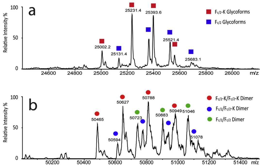
Fig. 5. Cetuximab Fc 1/2 variants deconvoluted mass spectra in (a) denaturing and (b) CZE conditions. Experimental conditions: denaturing conditions, 50%/49%/1%, acetonitrile/water/formic acid (v/v/v); CZE conditions, ammonium acetate 25 mM, pH 5.7; sample concentration 1 \mu M.
