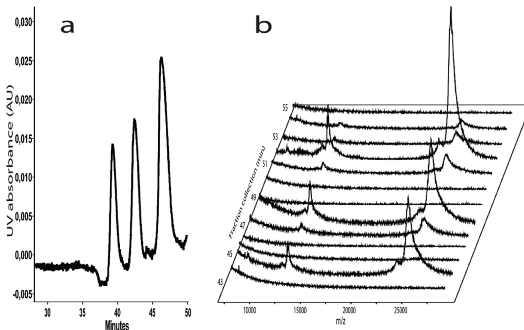
Fig. 2. CZE-UV off-line coupled to MALDI-MS via fractionation for a middle-up characterization of Cetuximab F_{c1/2} variants. (a) CZE-UV electropherogram. (b) Analysis of CZE-UV fractions by MALDI-MS. CE Experimental conditions: See Fig. 1; MS condition: See Experimental section; sample, IdeS digest of cetuximab (5 \mu\text{g}/\mu\text{L} ).
