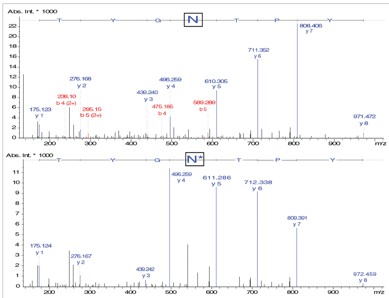
Figure 5. MS/MS spectra of peptide HT04 (IYPTNGYTR) (A) without modification and (B) with a deamidation on Asn 55 illustrating the partial modification of the mAb and the characterization of both forms by CESI-MS/MS. Experimental conditions: see Materials and Methods.
