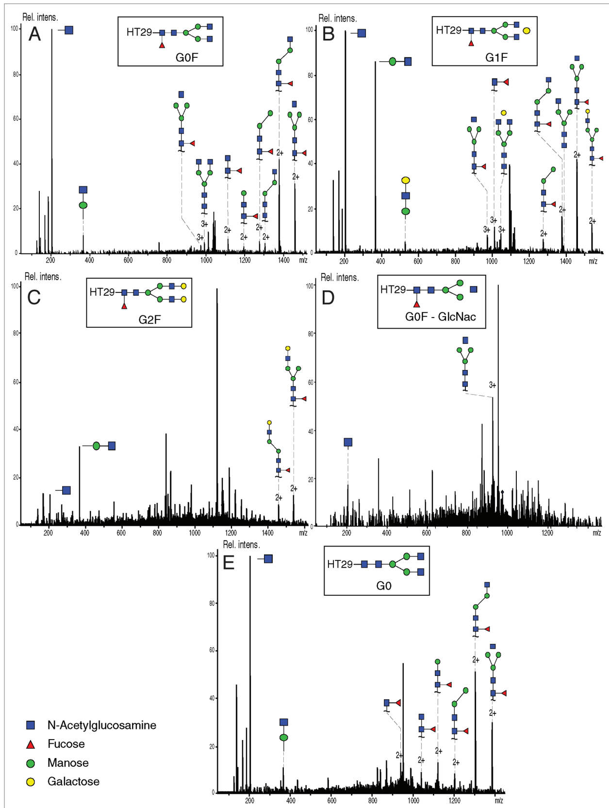
Figure 7. MS/MS fragmentation spectra of (A) HT29 - G0F (precursor m/z 1039.78; charge state 3+), (B) HT29 - G1F (precursor ion 1093.80; charge state 3+), (C) HT29 - G2F (precursor ion 1147.82; charge state 3+), (D) HT29 - G0F-GlcNAc (precursor ion 972.10; 3+), (E) HT29 - G0 (precursor ion 991.09; charge state 3+). Experimental conditions described in Materials and Methods section.
