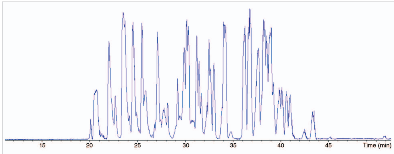
Figure 1. Base Peak Electropherogram corresponding to the analysis by CESI-MS/MS of trastuzumab tryptic digest. Experimental conditions: bare fused silica capillary with porous tip, total length 95 cm (30 \mu\text{m} i.d., 150 \mu\text{m} o.d.); CE voltage +20 kV; BGE 10% acetic acid; sample trastuzumab tryptic digest 2.5 mg/mL in BGE (11 nL injected). MS capillary voltage: -1.3 kV, m/z range: 50–3000.
