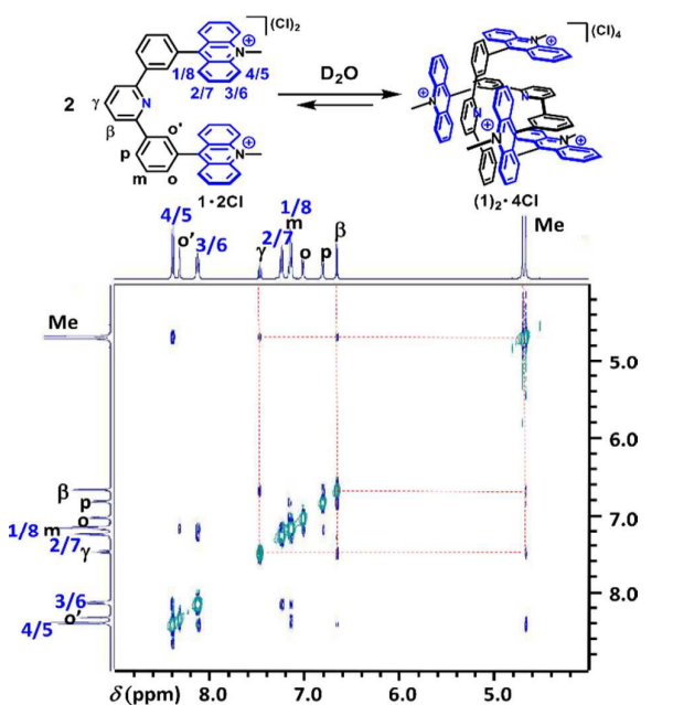
Fig. 4 ^1\text{H} - ^1\text{H} NOESY (500 MHz, \text{D}_2\text{O} , 298 K, c = 5 \cdot 10^{-3} \text{ mol L}^{-1} ) spectrum of (1)_2 \cdot 4\text{Cl} . Correlations between the \beta and \gamma protons of the pyridine with the methyl protons.
