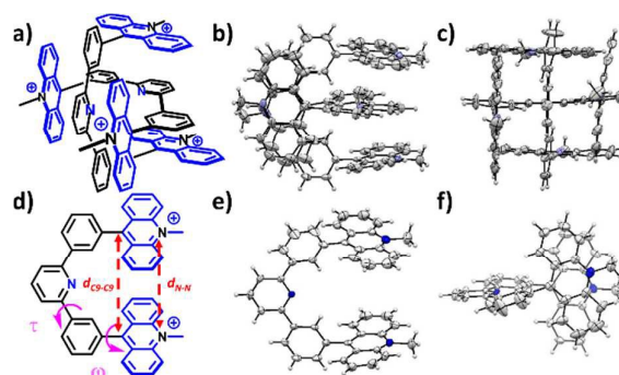
Fig. 3 Crystal structure views b-c and e-f of (1)_2\cdot 4\text{PF}_6 . a) Scheme of the entwined dimer of 1\cdot 2\text{PF}_6 . b) Side view of the entwined dimer of 1\cdot 2\text{PF}_6 showing the \pi - \pi stacking between the acridinium moieties and the 2,6-diphenylpyridine spacer. c) Rear view of the entwined dimer. d) Scheme of a 1\cdot 2\text{PF}_6 monomer of (1)_2\cdot 4\text{PF}_6 . e) Side view of a 1\cdot 2\text{PF}_6 monomer of (1)_2\cdot 4\text{PF}_6 showing the U-shaped conformation. f) Top view of a 1\cdot 2\text{PF}_6 monomer of (1)_2\cdot 4\text{PF}_6 .
