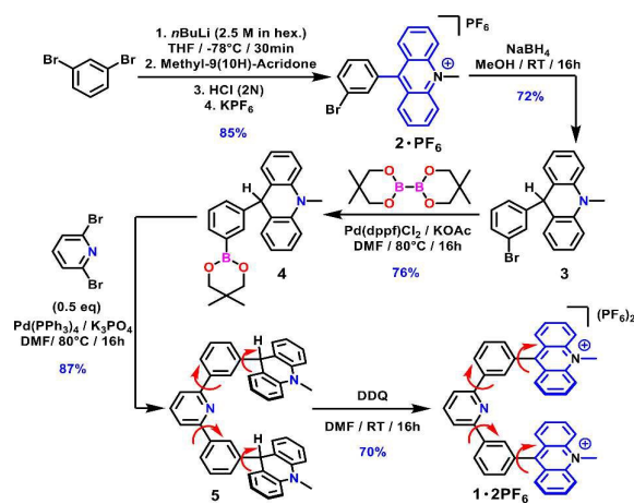
Scheme 1 Synthesis of 1·2PF 6 from 1,3-dibromobenzene as starting material.
