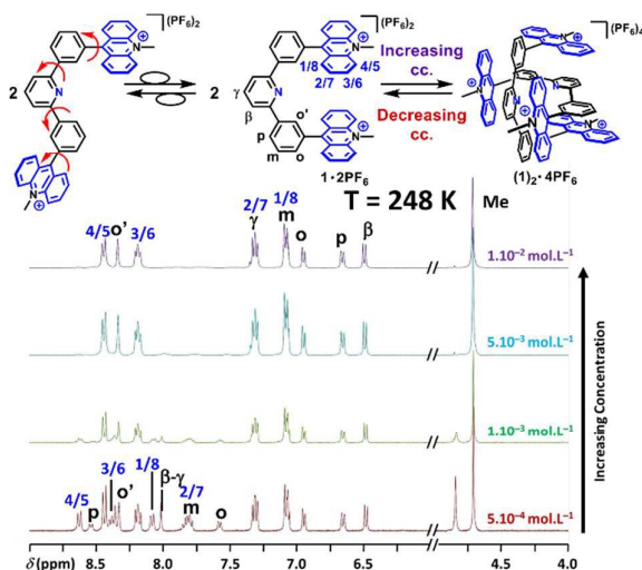
Fig. 2 ^1\text{H} NMR (500 MHz, \text{CD}_3\text{CN} , 248 K) spectra of 1\cdot 2\text{PF}_6 at 1\cdot 10^{-2} , 5\cdot 10^{-3} , 1\cdot 10^{-3} and 5\cdot 10^{-4} \text{mol}\cdot\text{L}^{-1} . At 1\cdot 10^{-2} \text{mol}\cdot\text{L}^{-1} , the assignments correspond to the protons of the dimer (1)_2\cdot 4\text{PF}_6 . At 5\cdot 10^{-4} \text{mol}\cdot\text{L}^{-1} , the dimer-monomer ratio is 7:3 and only the assignments of the protons of the monomeric species is shown.
